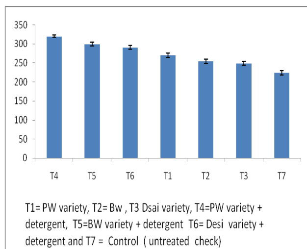
Figure 1. Average yield of cabbage crop per plot.
